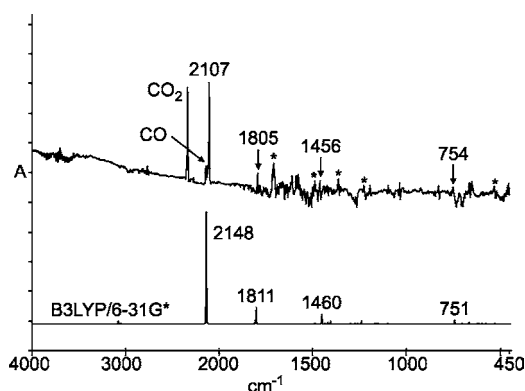
Figure 1. Measured and calculated (B3LYP/6-31G*) IR spectra of cyclopropabenzylidenethenone 12 ; * = peaks due to acetone [Supporting Information contains computational coordinates, energies, and a full-scale IR spectrum].
